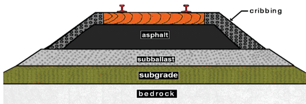
Fig 5: Ballastless trackbed containing thickened asphalt and subballast layers (used in Japan)
