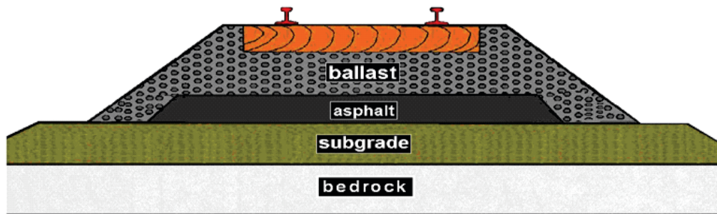
Fig 3: Asphalt Underlayment trackbed without granular subballast layer (common in USA)
