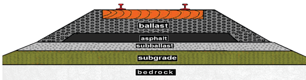
Fig 4: Asphalt Combination trackbed containing both asphalt and subballast layers (common in Europe and Asia)
