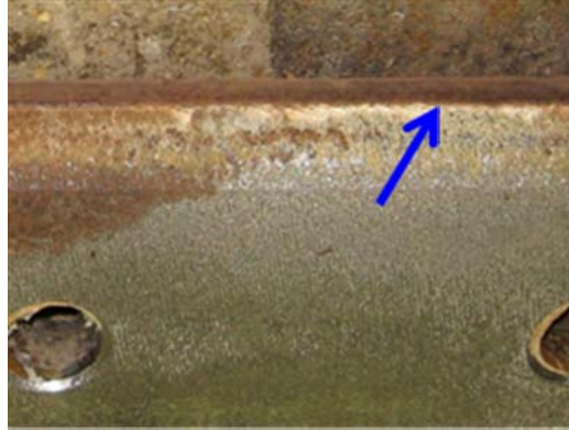
Figure 4: Debonding behind visible edge of insulator without corresponding debonding on hidden surface.
