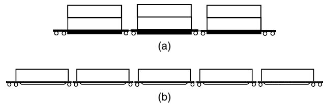
Figure 1 (a) A Three-Unit Well Car with Six Slots and (b) A Five-Unit Spine Car with Five Slots
