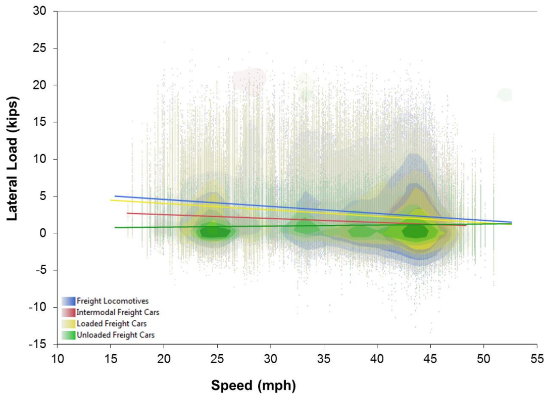
FIGURE 7 Lateral load variation with speed: low rail.
