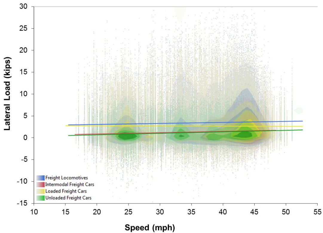
FIGURE 6 Lateral load variation with speed: high rail.
