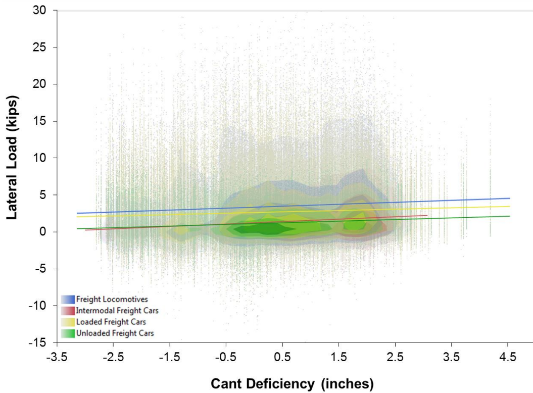
FIGURE 8 Lateral load variation with cant deficiency: high rail.
