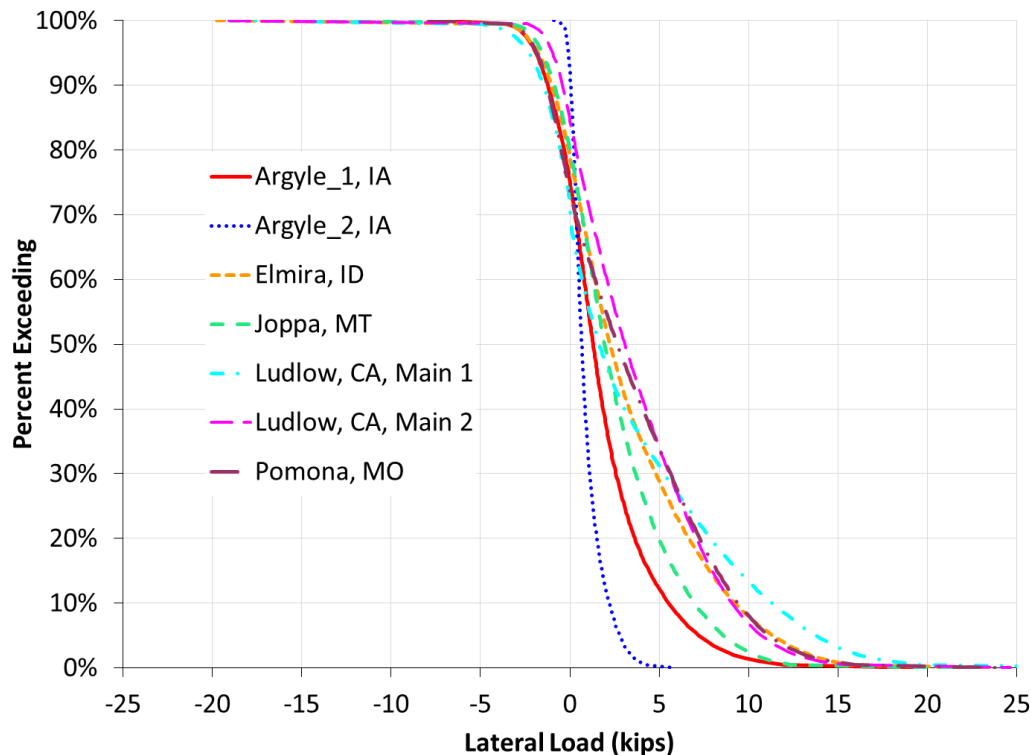
FIGURE 11 Lateral load variation with location: loaded freight cars.
