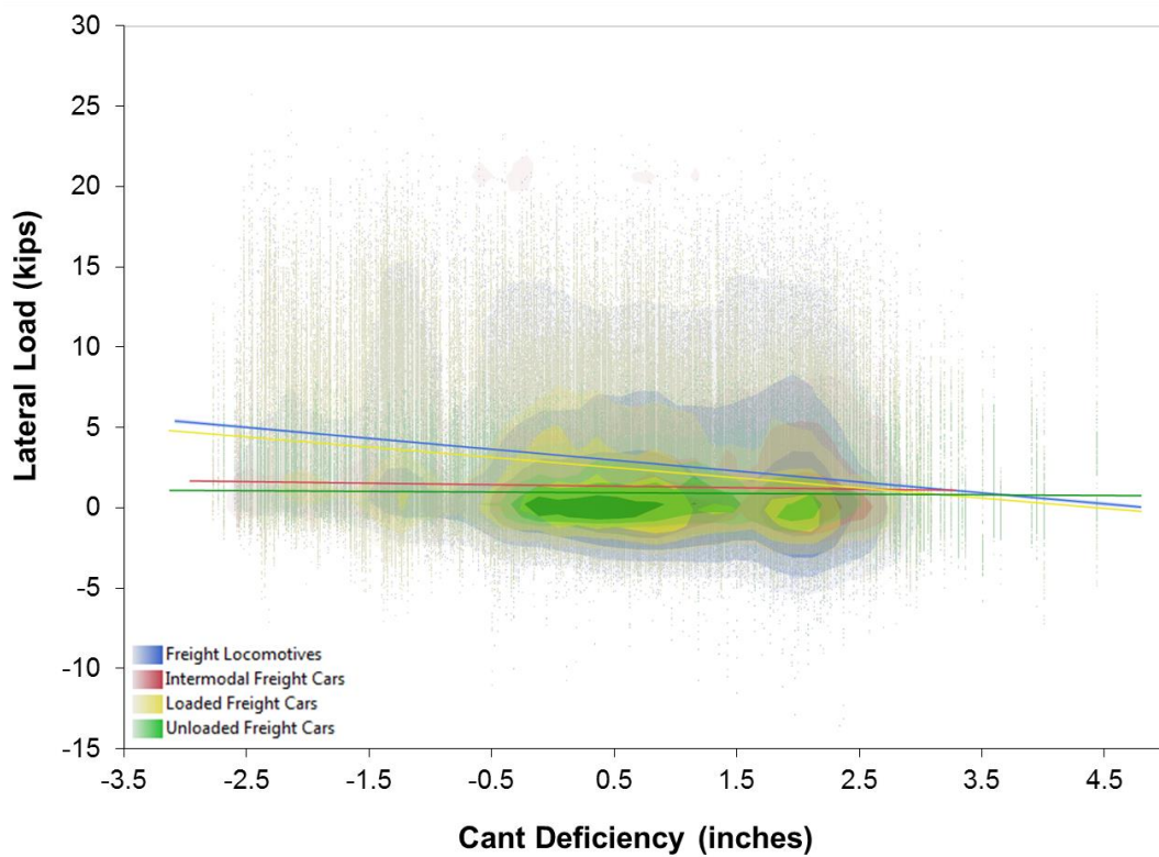
FIGURE 9 Lateral load variation with cant deficiency: low rail.
