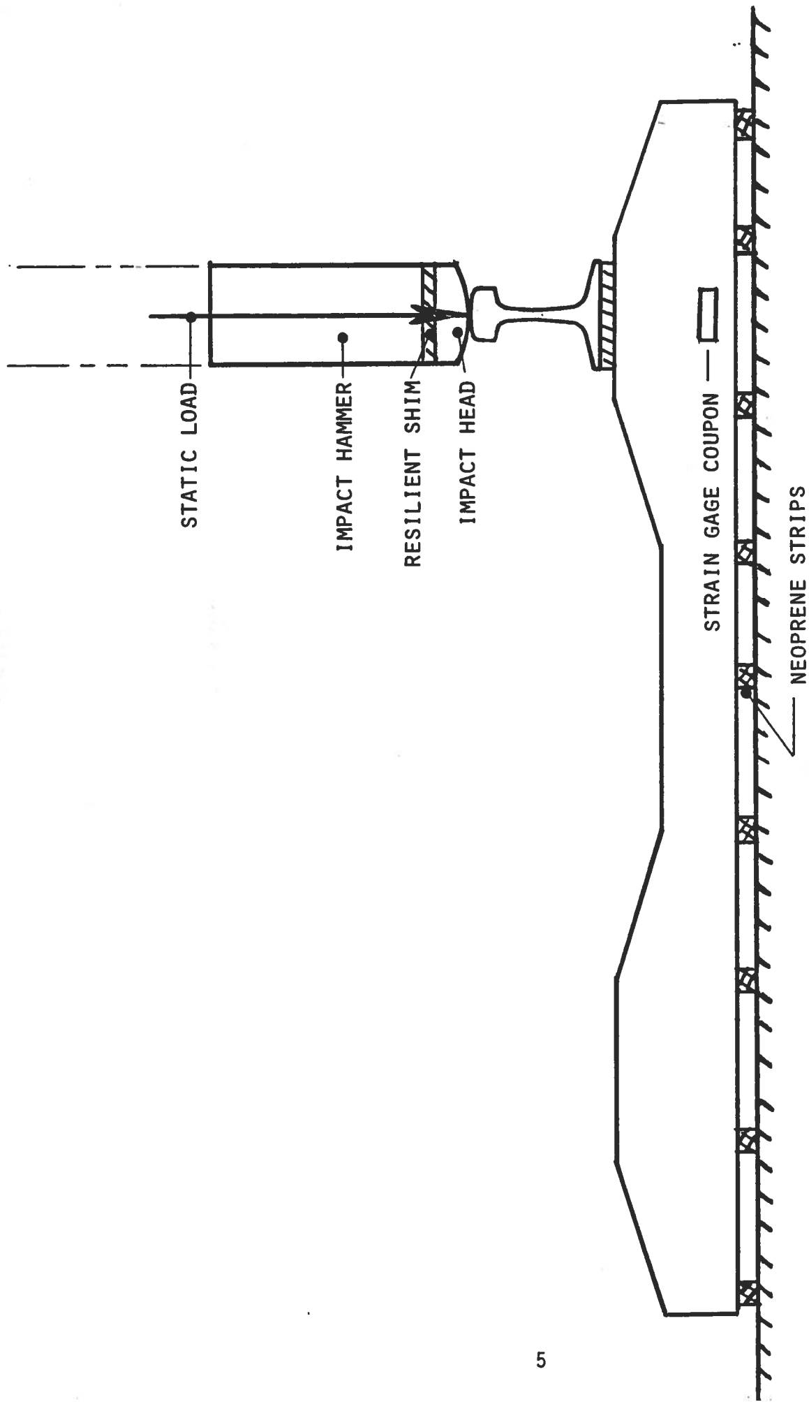
FIGURE 1. SCHEMATIC OF IMPACT TEST ARRANGEMENT
