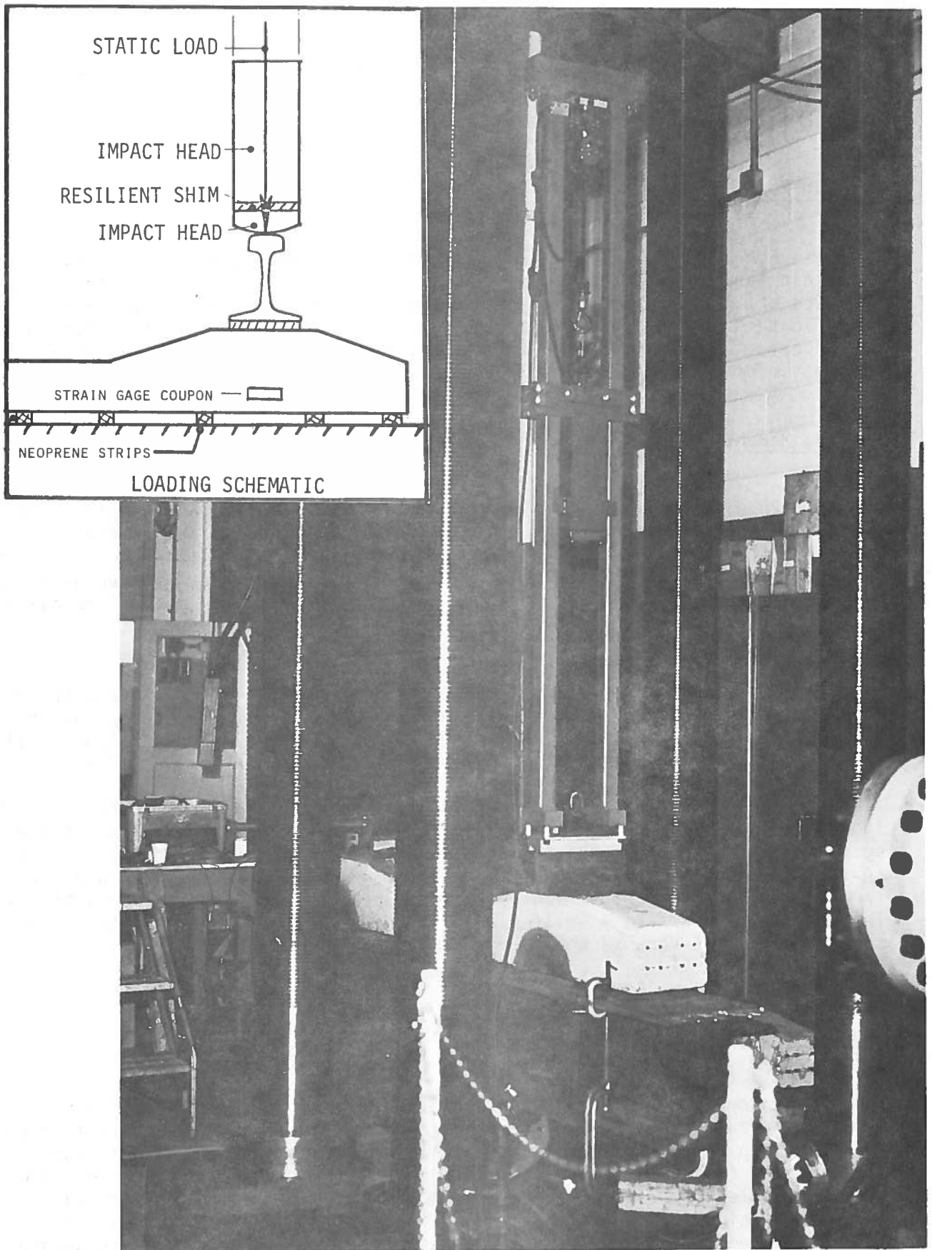
FIGURE 4-1. IMPACT LOADING FIXTURE
