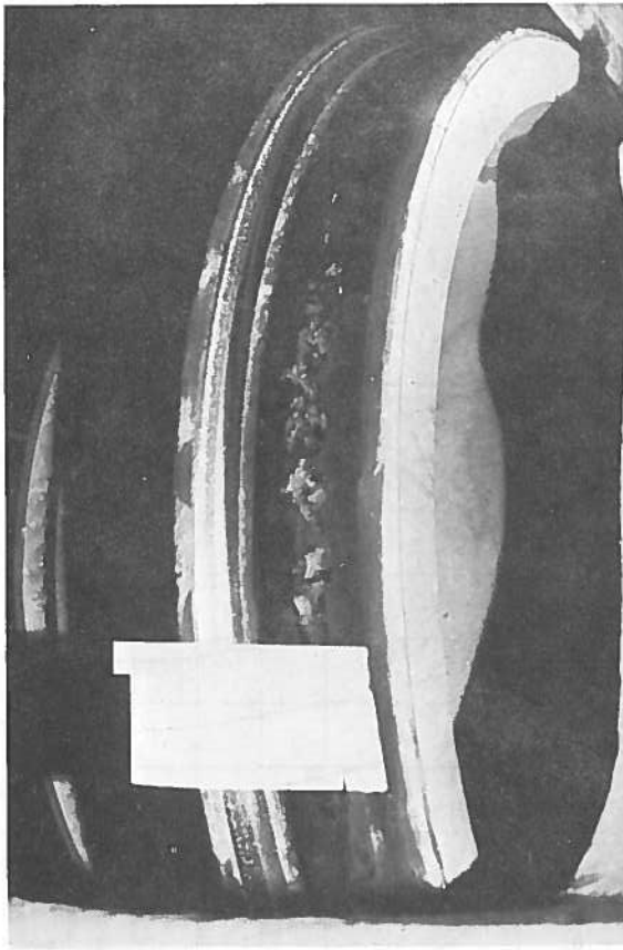
(a) Typical Spalled Wheel Tread
