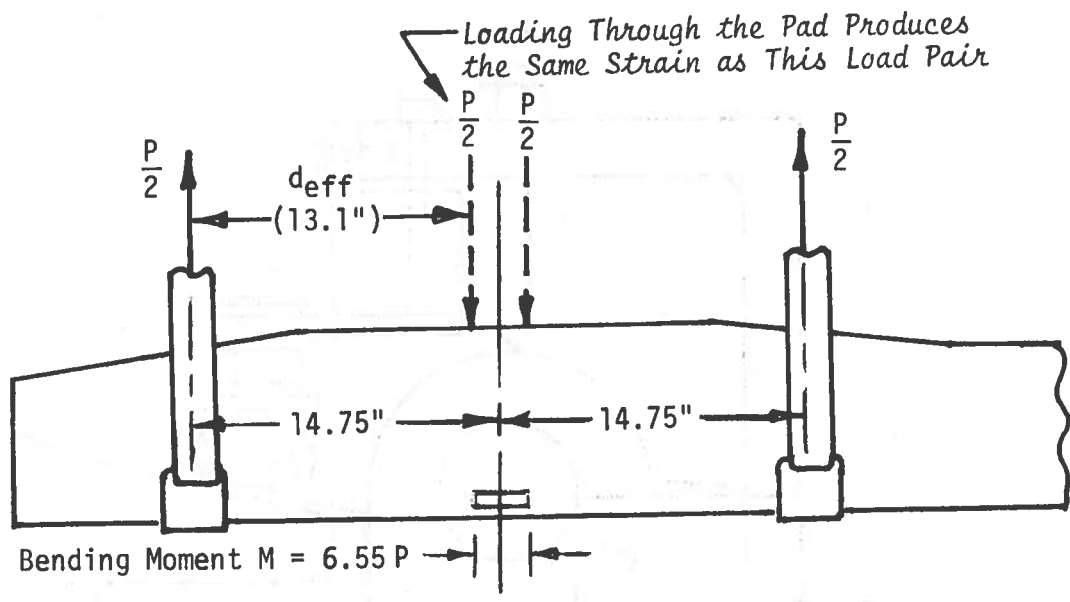
(b) Loading Schematic
