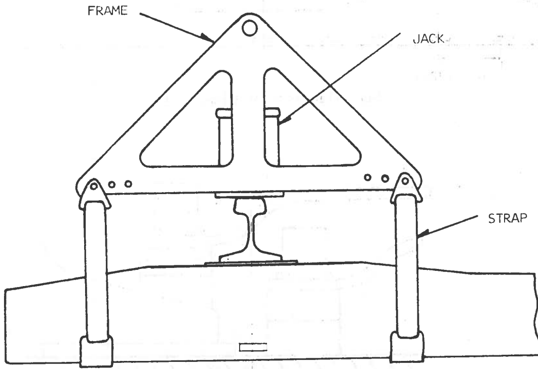
(a) Rail Seat Loading Arrangement
