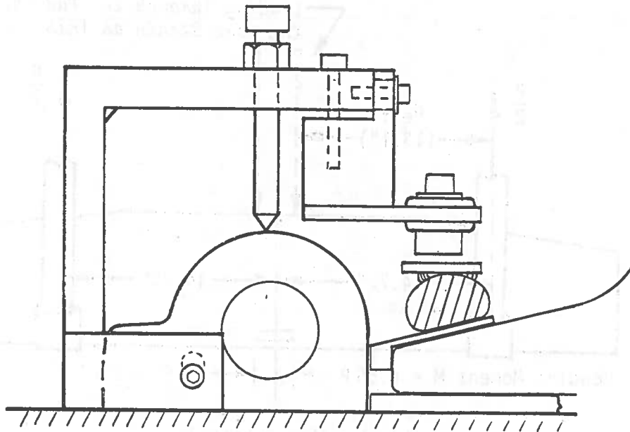
(c) Rail Clip Vertical Deflections
