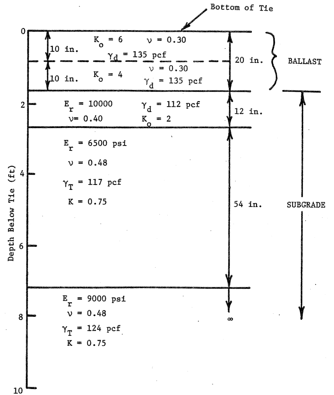
Figure 25. Layer Description for Aberdeen
