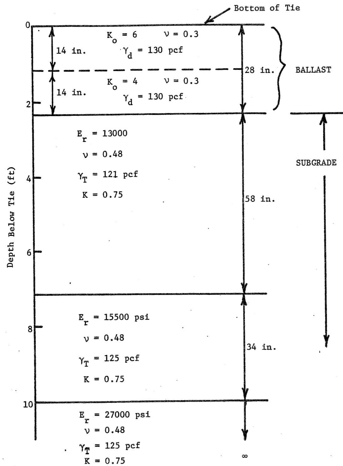
Figure 24. Layer Description for Lorraine
