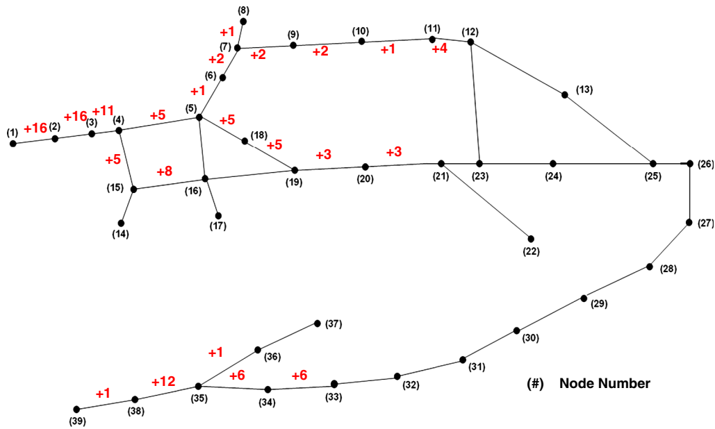
Fig. 8. Case study II network and the optimal solution
