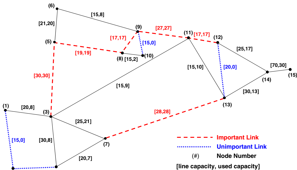
Fig. 7. Capacity usage of each link
